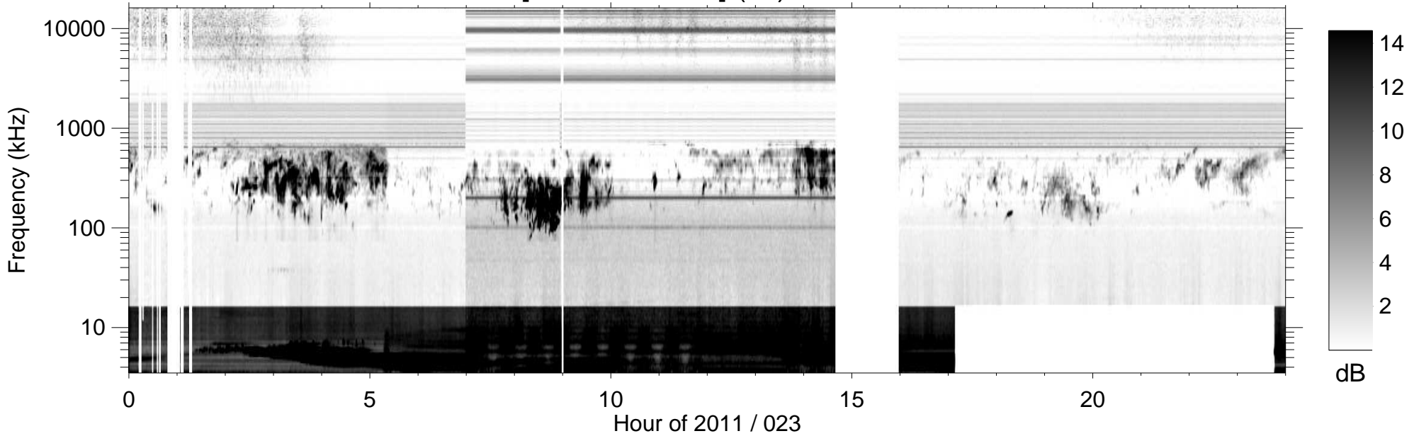
RPWS [ABCH1H2/Ex] (-B) 2011/01/23
