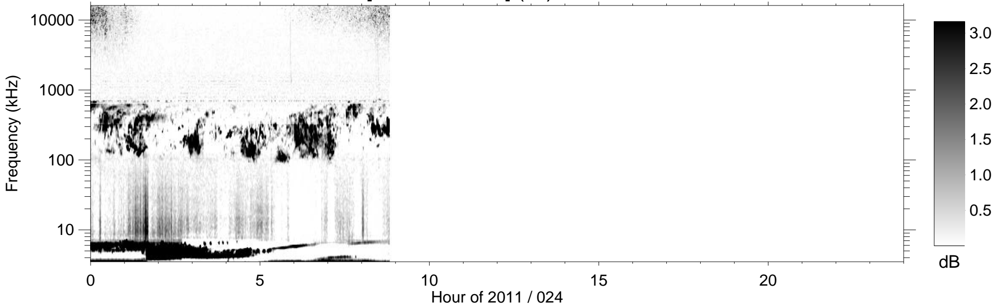
RPWS [ABCH1H2/Ex] (-B) 2011/01/24
