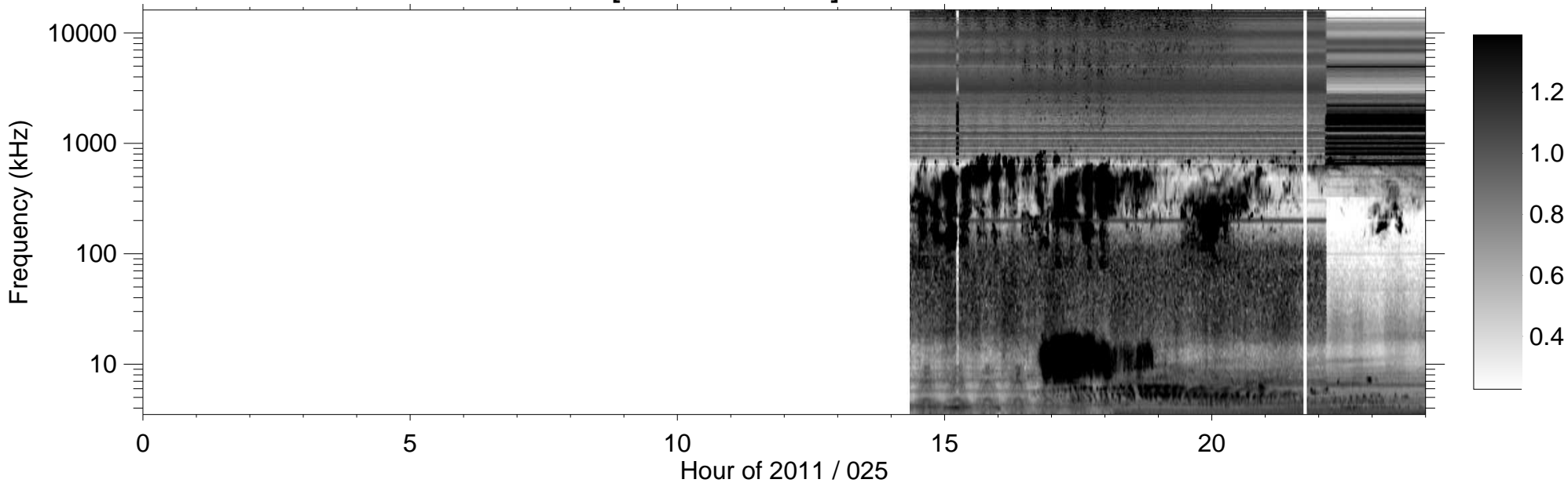
RPWS [ABCH1H2/Ex] (-B) 2011/01/25
