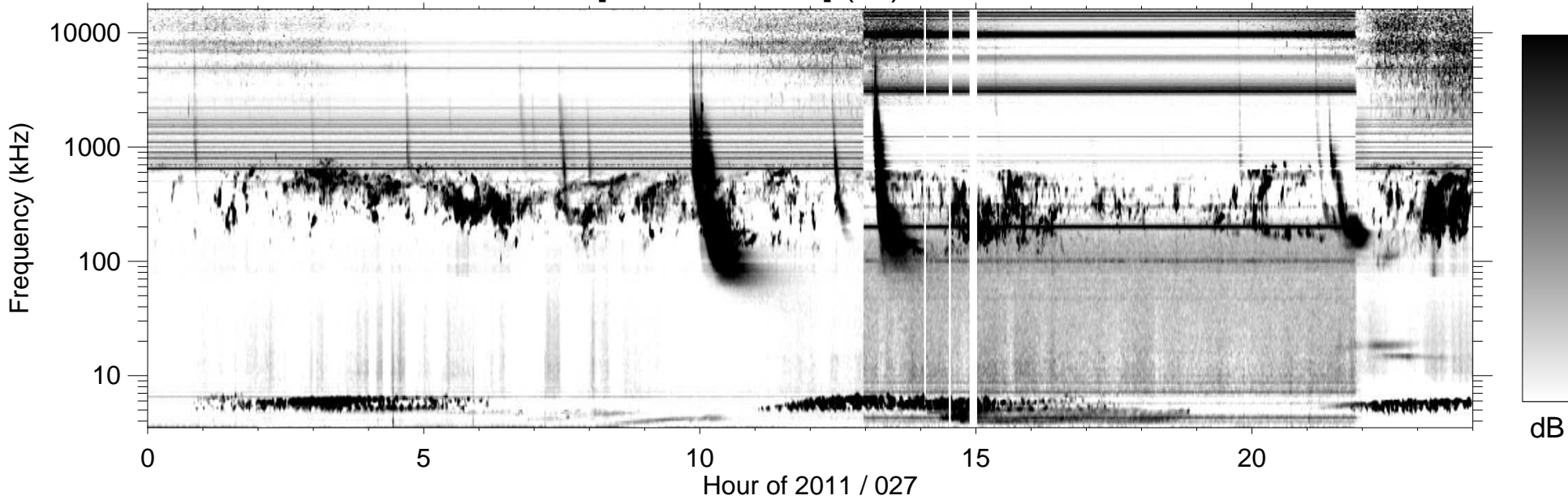
RPWS [ABCH1H2/Ex] (-B) 2011/01/27
