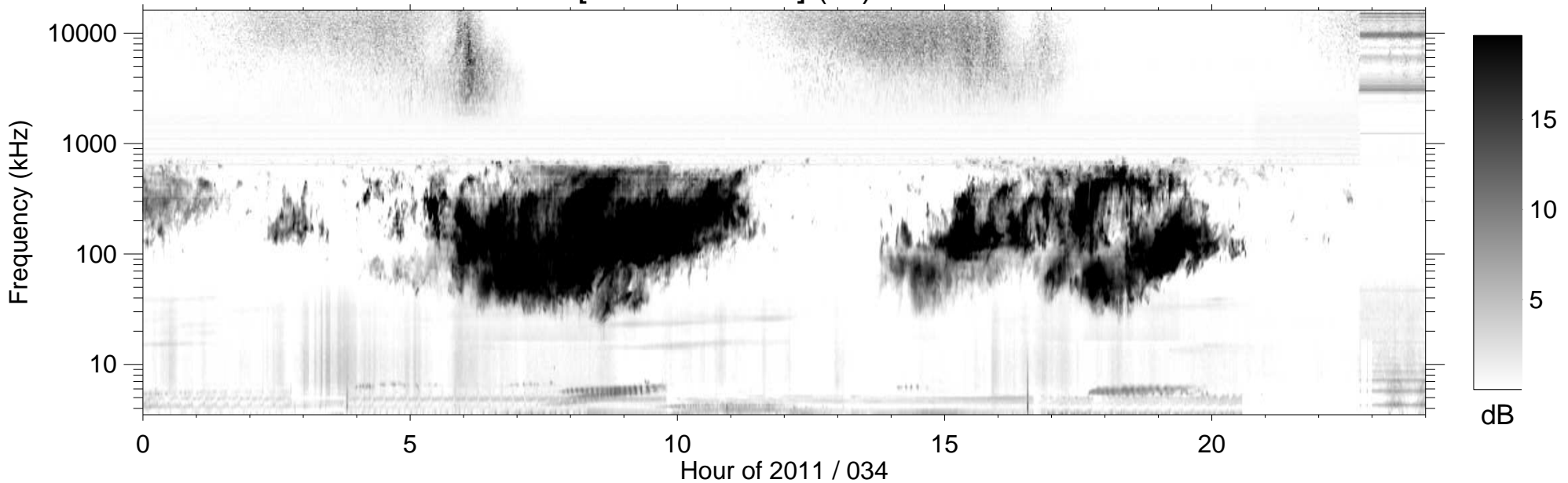
RPWS [ABCH1H2/Ex] (-B) 2011/02/03
