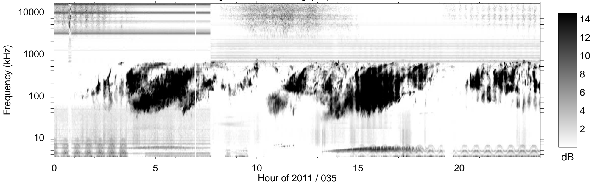
RPWS [ABCH1H2/Ex] (-B) 2011/02/04
