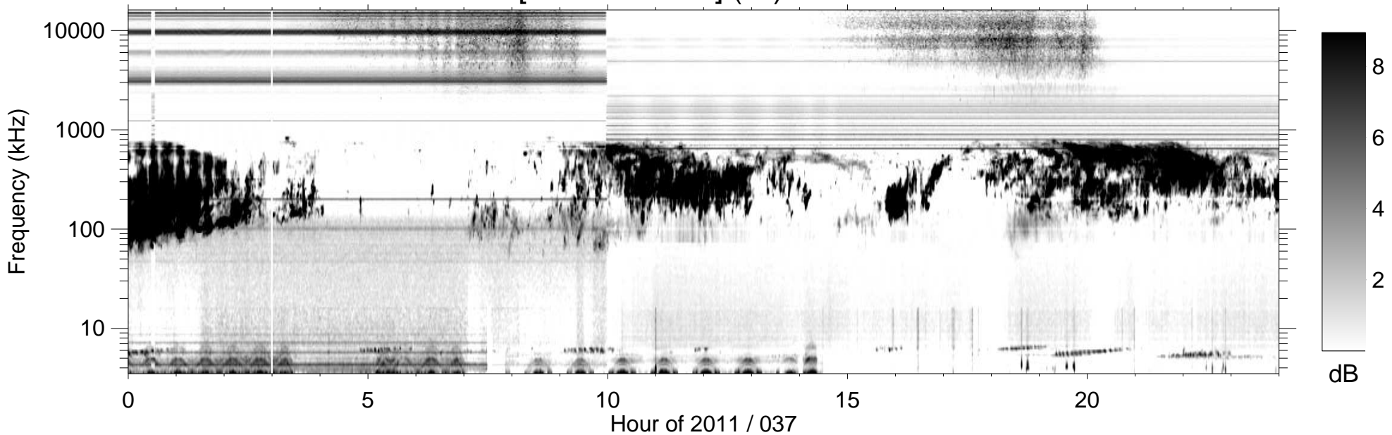
RPWS [ABCH1H2/Ex] (-B) 2011/02/06
