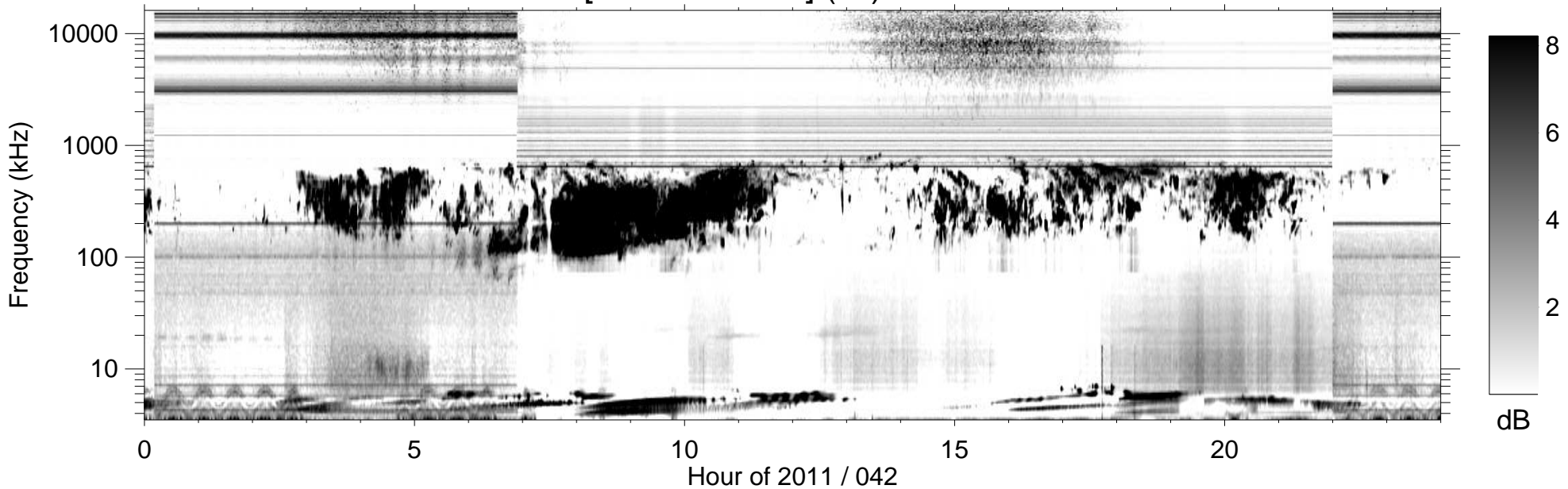
RPWS [ABCH1H2/Ex] (-B) 2011/02/11
