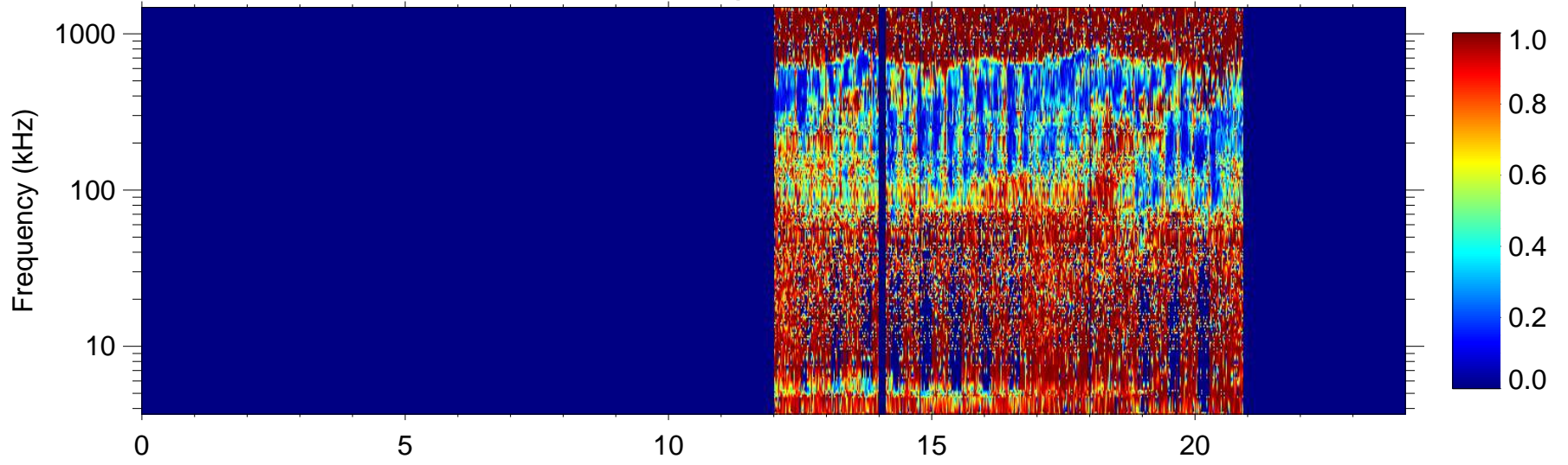
Total polarization
