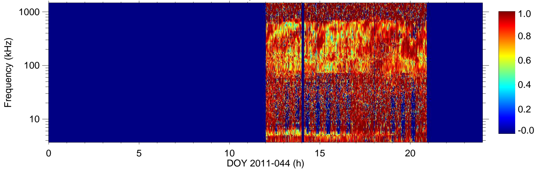
Total polarization
