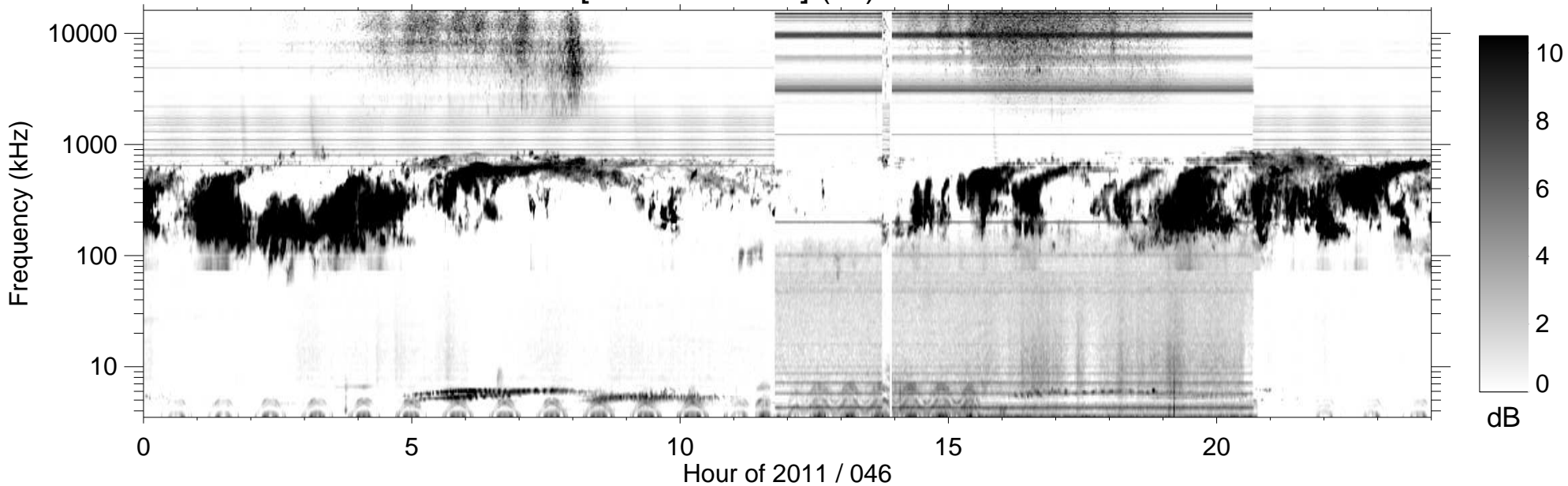
RPWS [ABCH1H2/Ex] (-B) 2011/02/15
