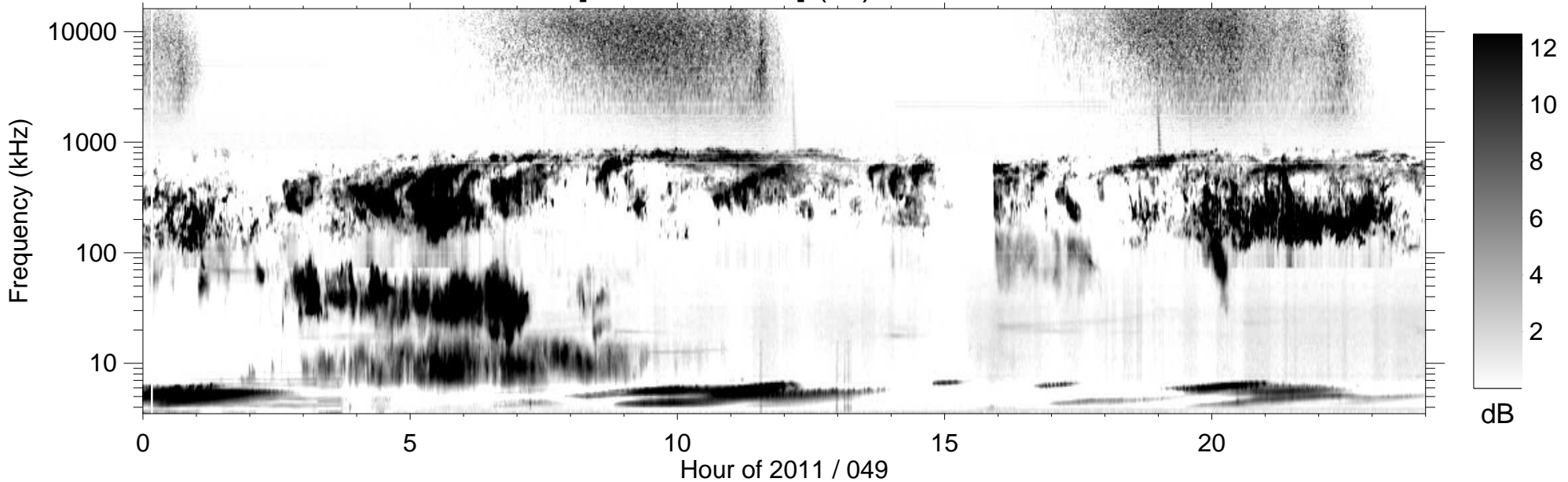
RPWS [ABCH1H2/Ex] (-B) 2011/02/18
