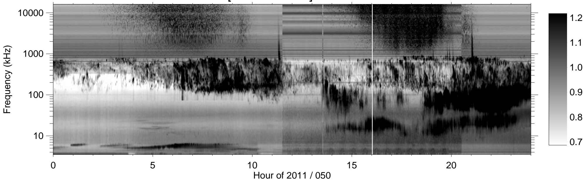
RPWS [ABCH1H2/Ex] (-B) 2011/02/19
