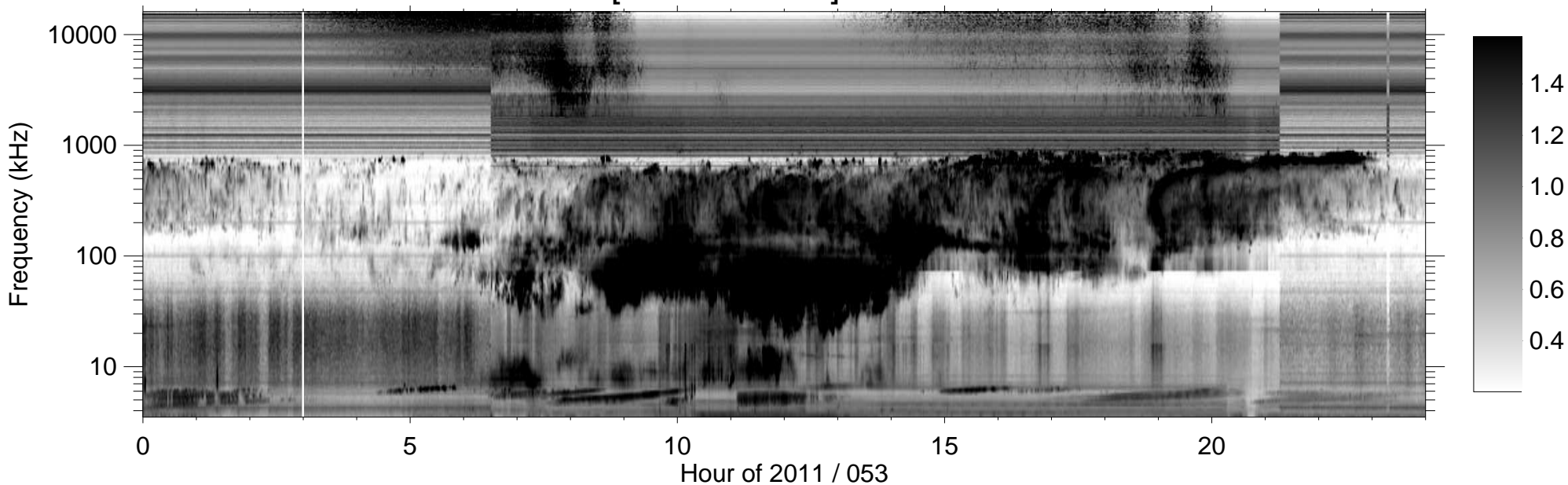
RPWS [ABCH1H2/Ex] (-B) 2011/02/22
