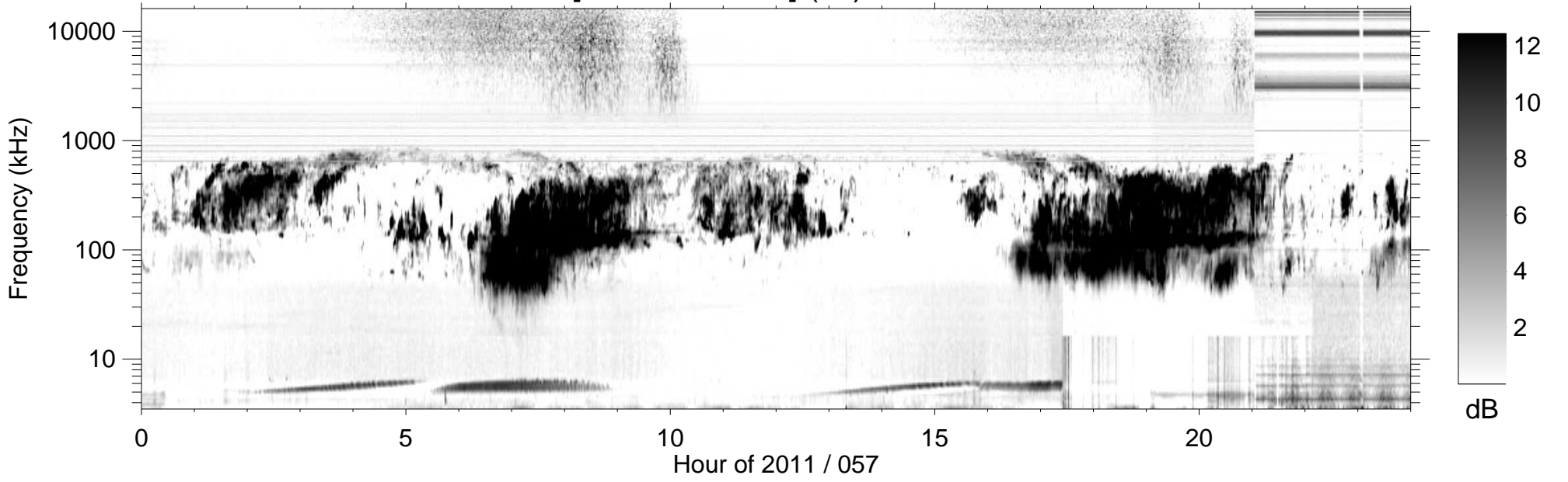
RPWS [ABCH1H2/Ex] (-B) 2011/02/26
