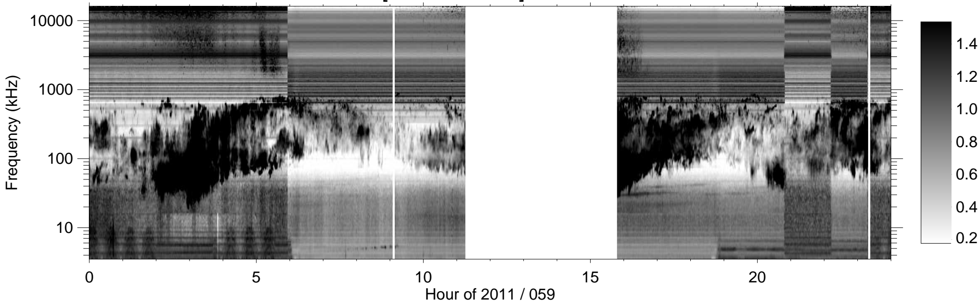
RPWS [ABCH1H2/Ex] (-B) 2011/02/28
