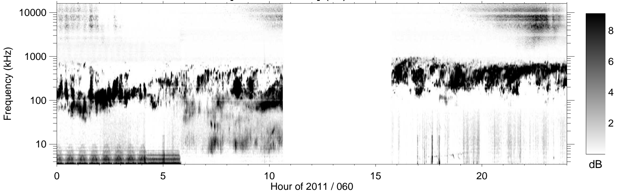
RPWS [ABCH1H2/Ex] (-B) 2011/03/01
