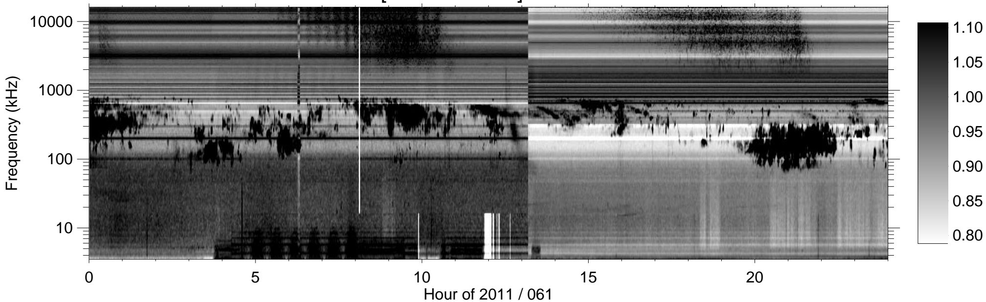
RPWS [ABCH1H2/Ex] (-B) 2011/03/02
