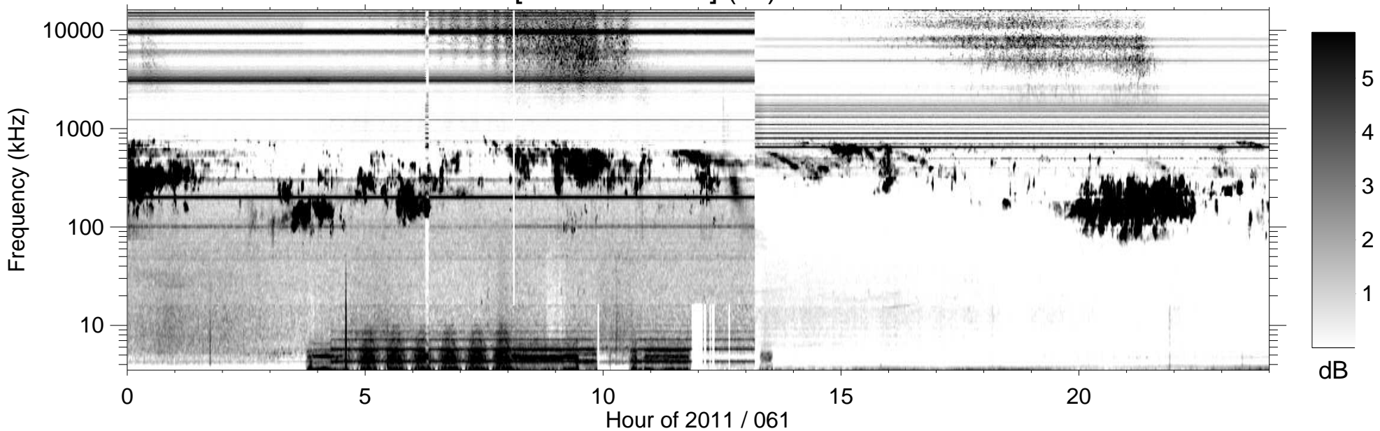
RPWS [ABCH1H2/Ex] (-B) 2011/03/02
