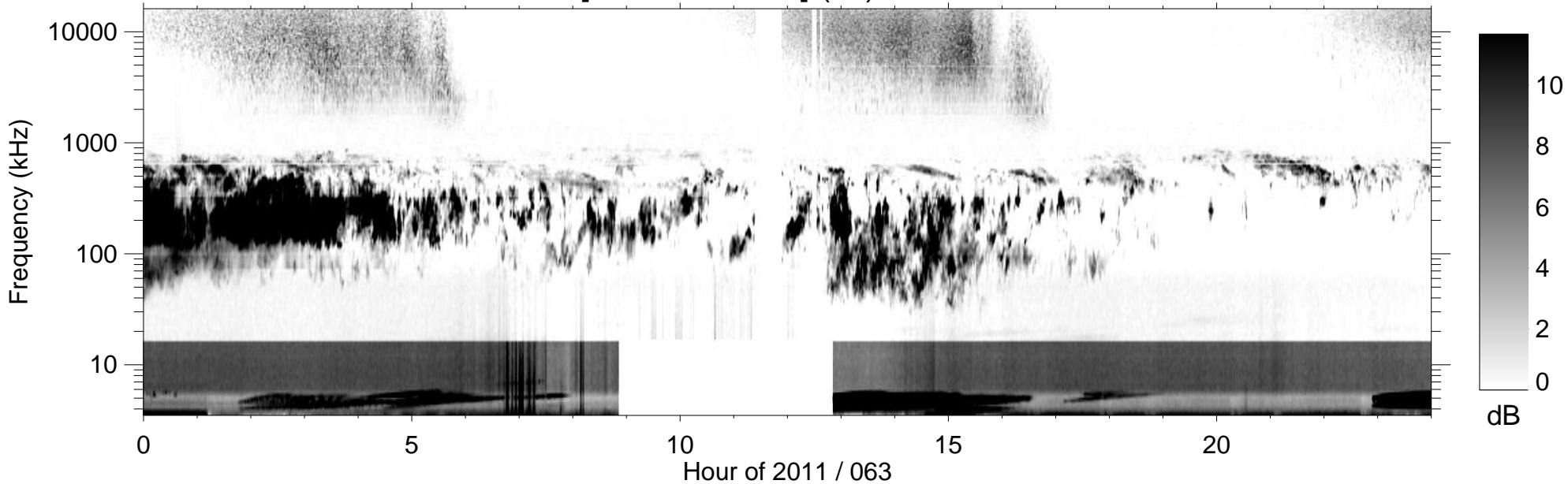
RPWS [ABCH1H2/Ex] (-B) 2011/03/04
