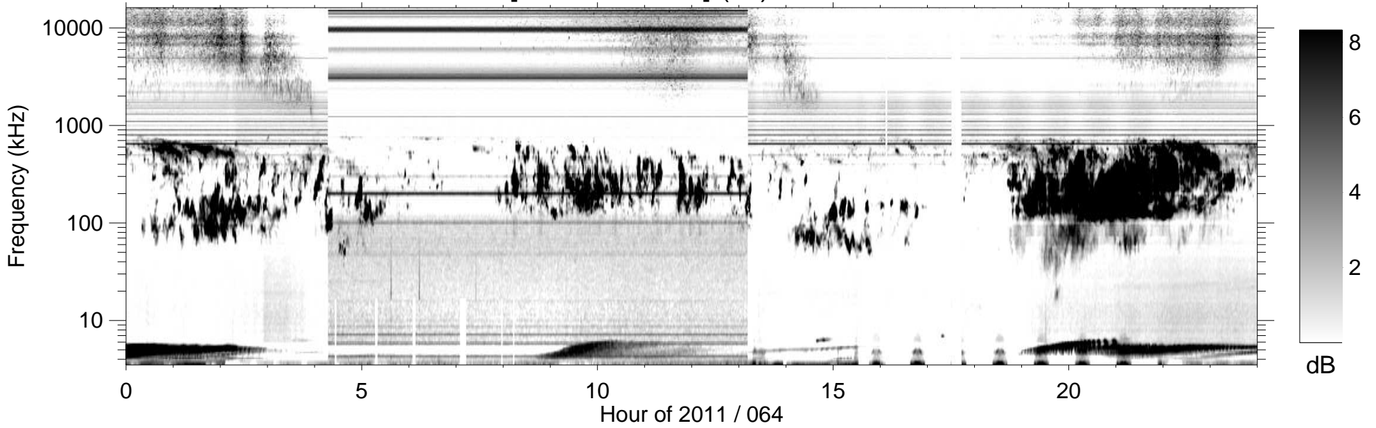
RPWS [ABCH1H2/Ex] (-B) 2011/03/05
