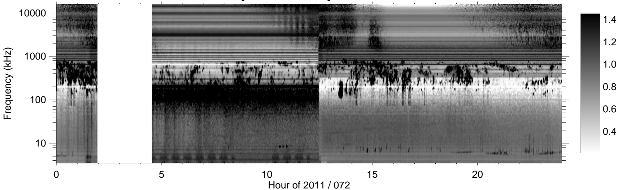
RPWS [ABCH1H2/Ex] (-B) 2011/03/13
