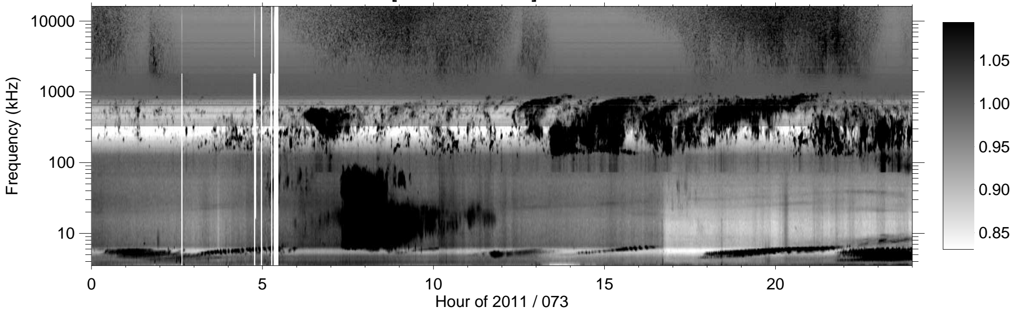
RPWS [ABCH1H2/Ex] (-B) 2011/03/14
