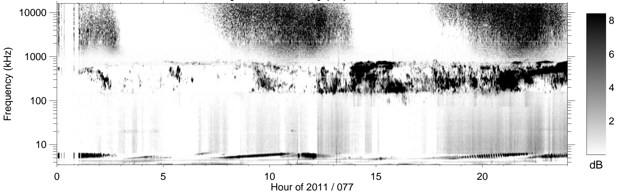
RPWS [ABCH1H2/Ex] (-B) 2011/03/18
