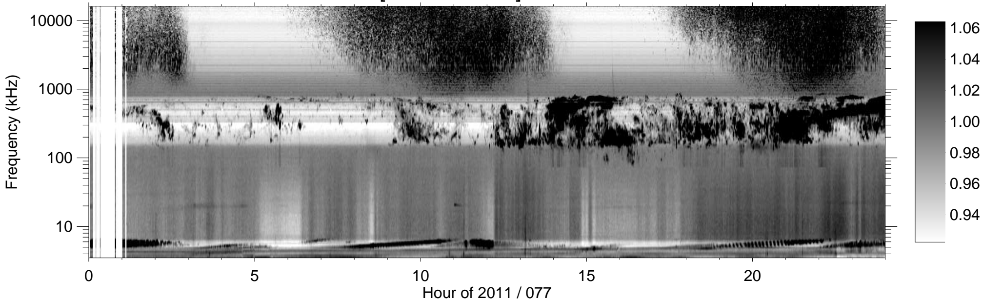
RPWS [ABCH1H2/Ex] (-B) 2011/03/18
