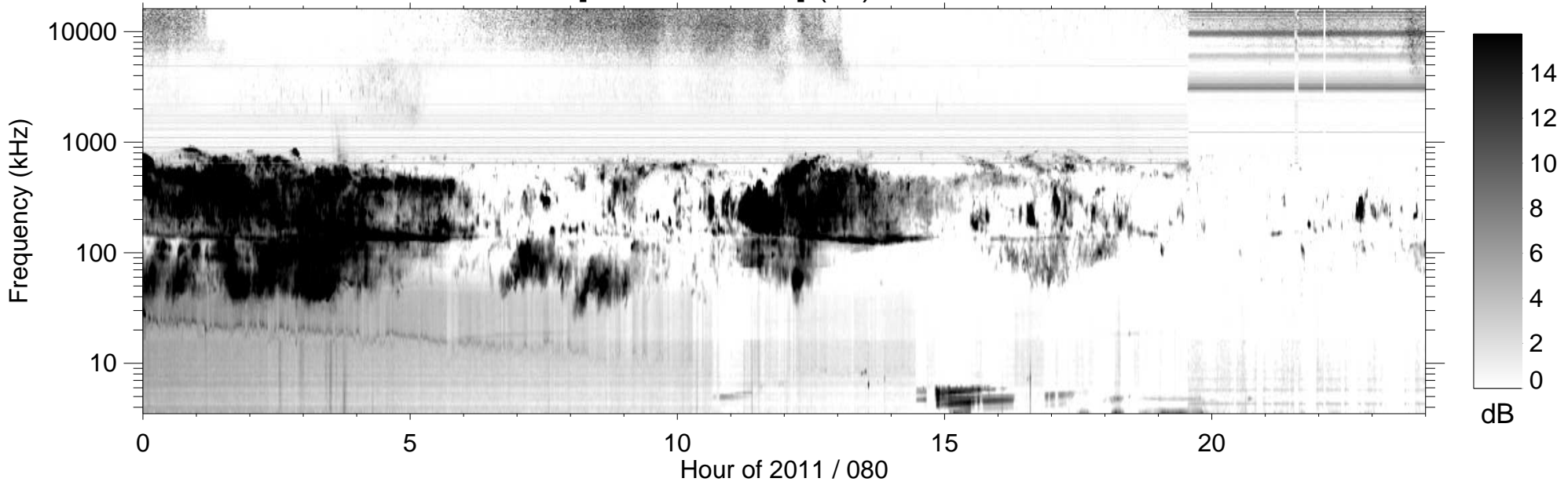
RPWS [ABCH1H2/Ex] (-B) 2011/03/21
