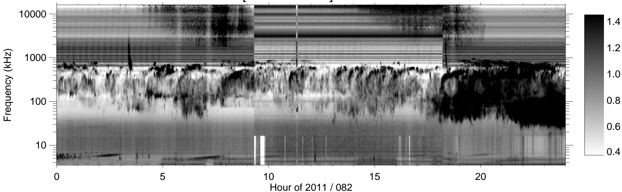
RPWS [ABCH1H2/Ex] (-B) 2011/03/23
