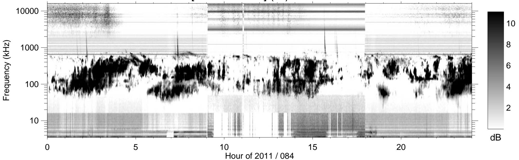
RPWS [ABCH1H2/Ex] (-B) 2011/03/25
