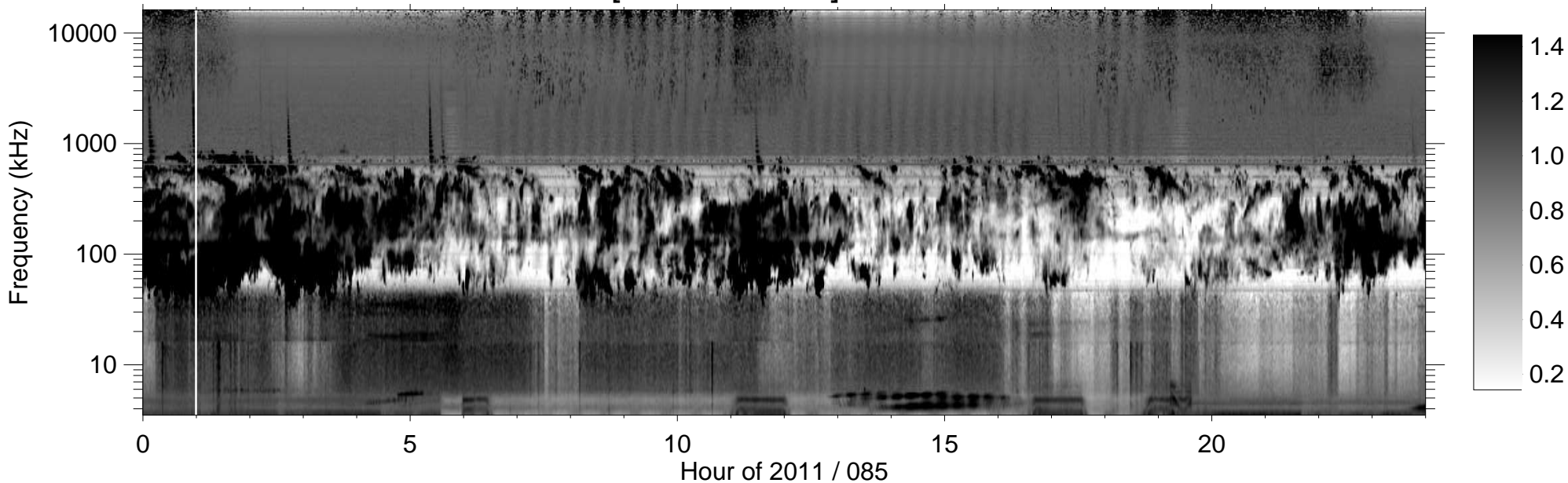
RPWS [ABCH1H2/Ex] (-B) 2011/03/26
