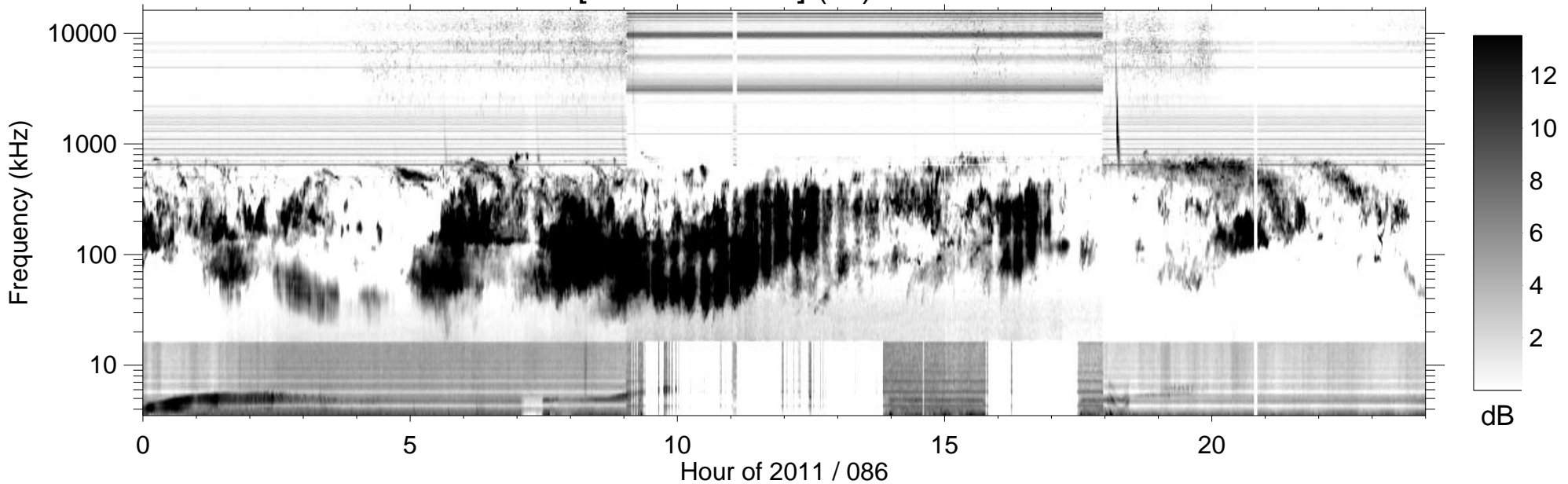
RPWS [ABCH1H2/Ex] (-B) 2011/03/27
