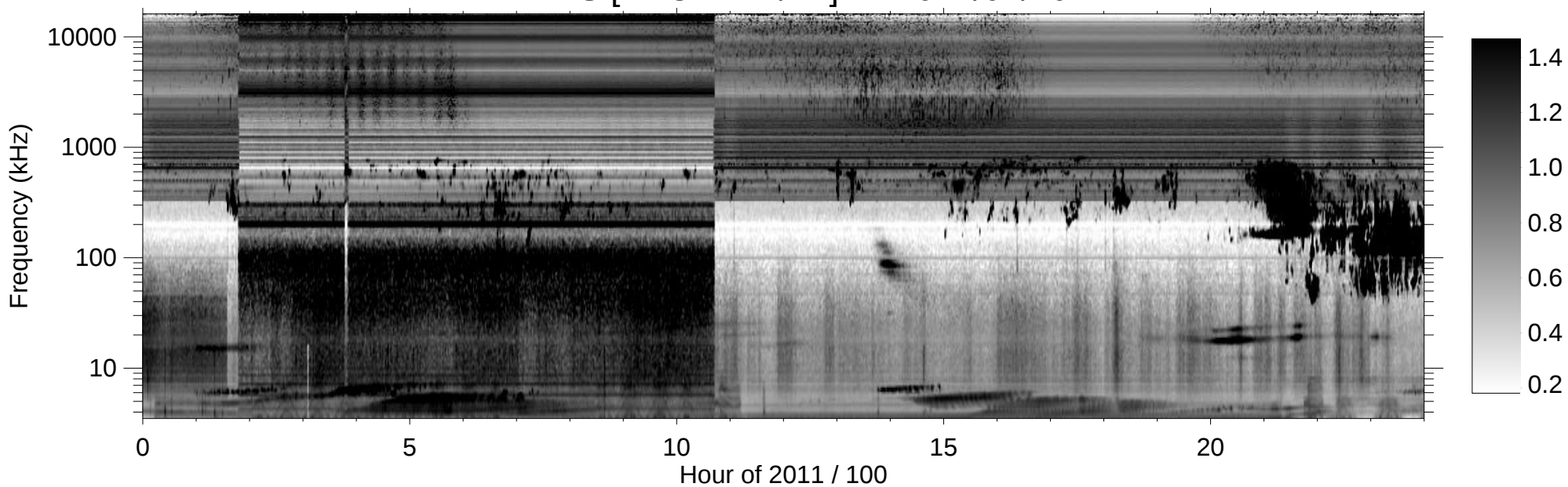
RPWS [ABCH1H2/Ex] (-B) 2011/04/10
