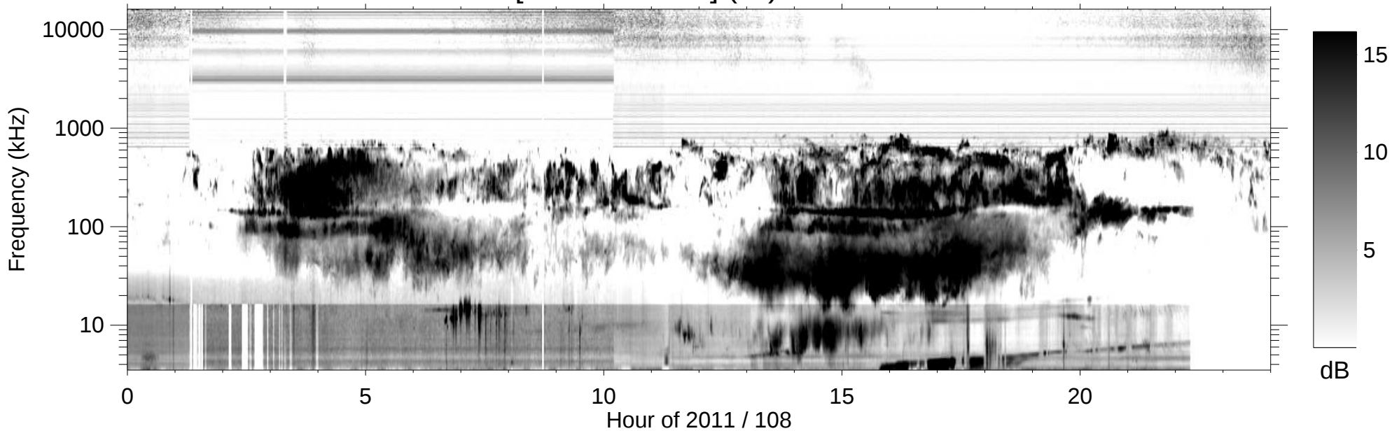
RPWS [ABCH1H2/Ex] (-B) 2011/04/18
