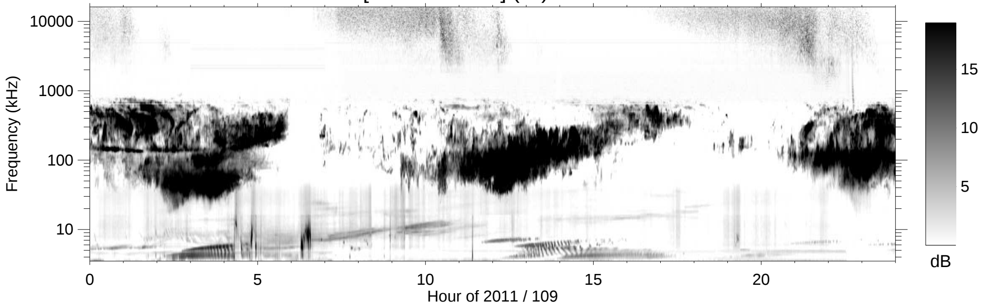
RPWS [ABCH1H2/Ex] (-B) 2011/04/19
