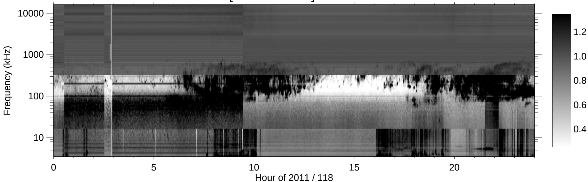
RPWS [ABCH1H2/Ex] (-B) 2011/04/28
