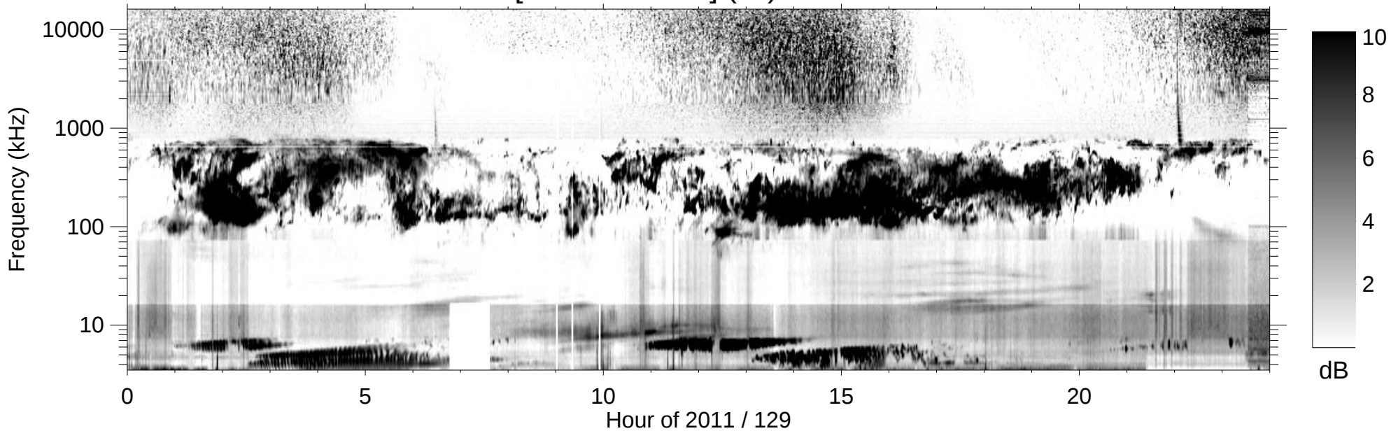
RPWS [ABCH1H2/Ex] (-B) 2011/05/09
