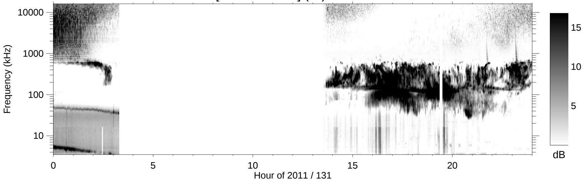
RPWS [ABCH1H2/Ex] (-B) 2011/05/11
