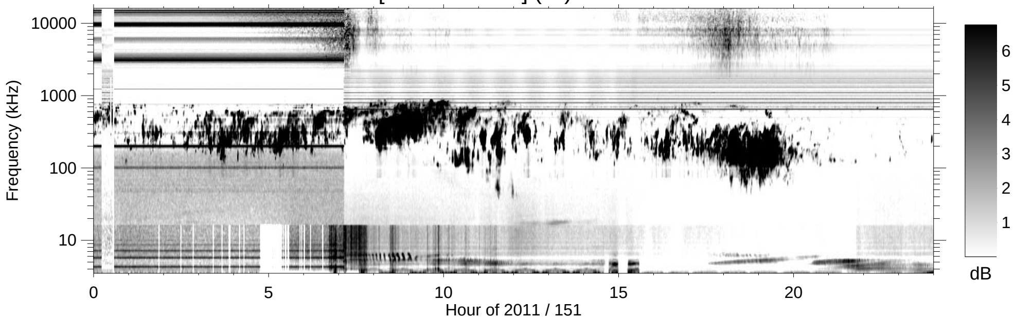
RPWS [ABCH1H2/Ex] (-B) 2011/05/31
