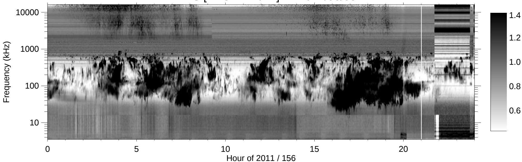
RPWS [ABCH1H2/Ex] (-B) 2011/06/05
