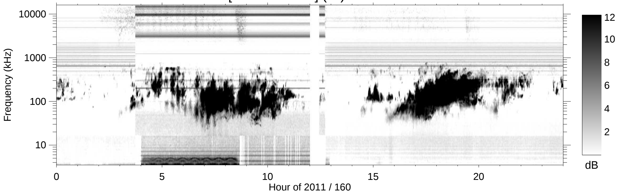
RPWS [ABCH1H2/Ex] (-B) 2011/06/09
