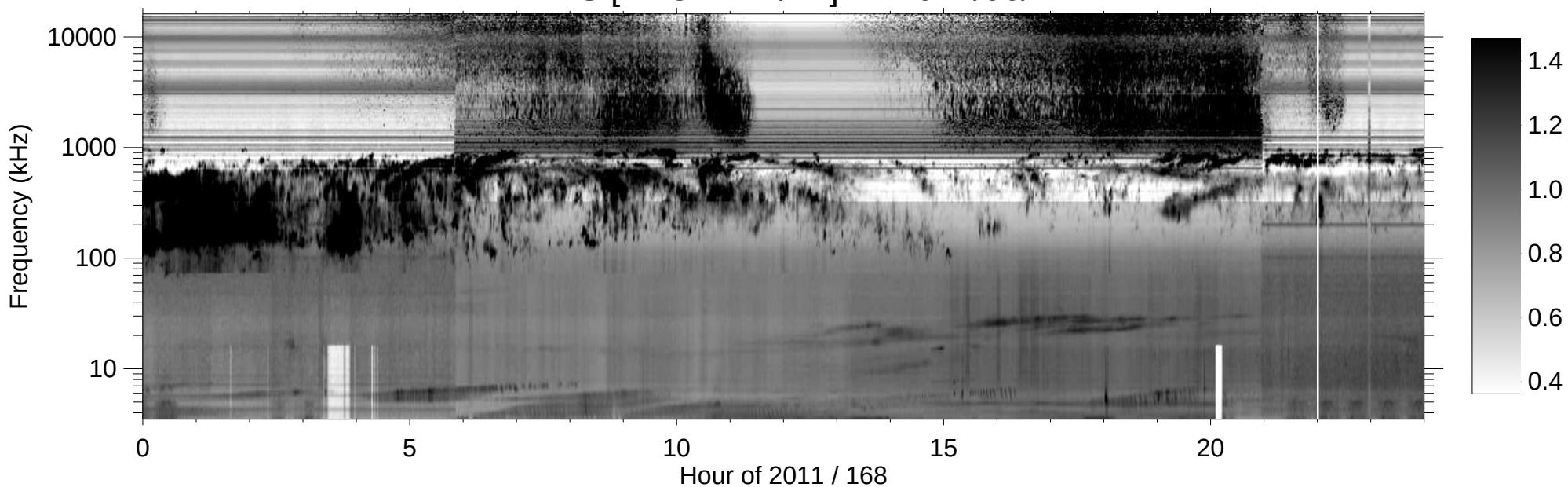
RPWS [ABCH1H2/Ex] (-B) 2011/06/17
