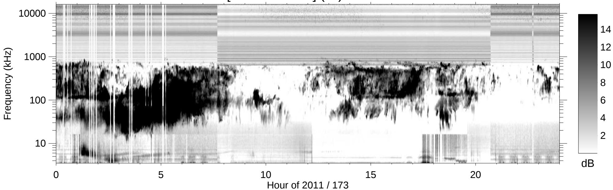
RPWS [ABCH1H2/Ex] (-B) 2011/06/22
