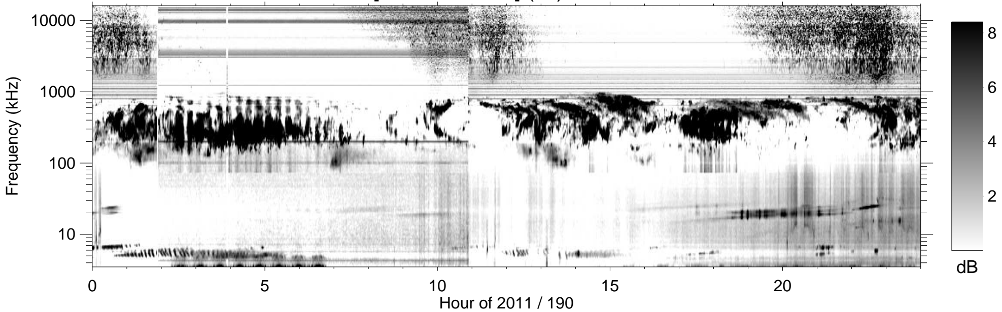
RPWS [ABCH1H2/Ex] (-B) 2011/07/09
