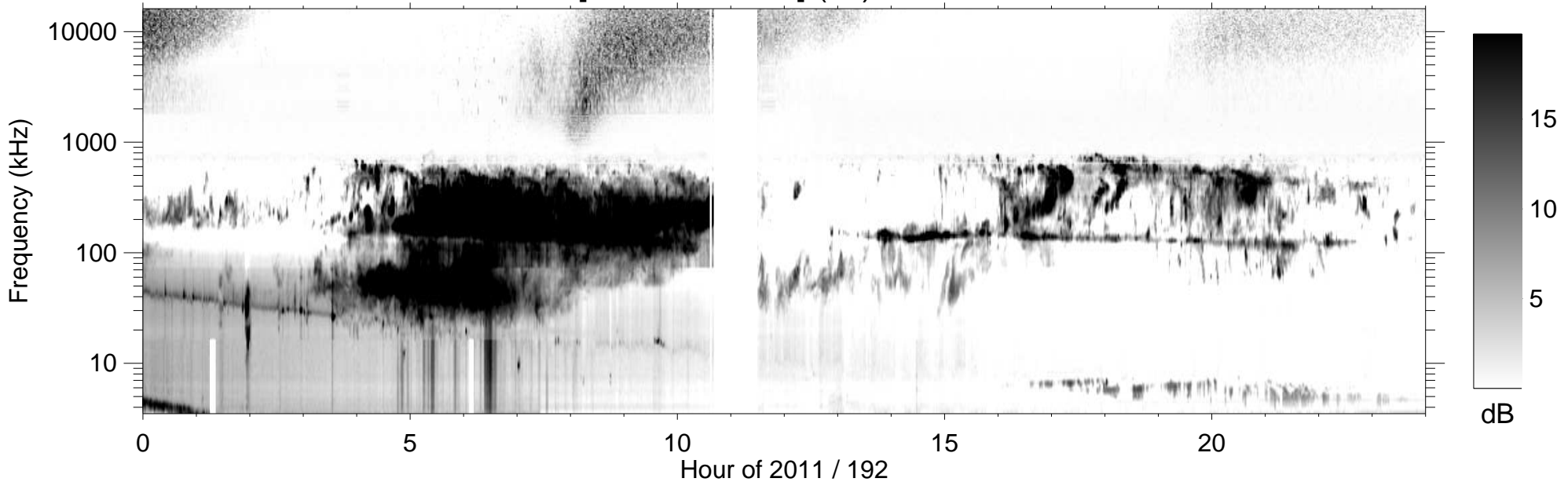
RPWS [ABCH1H2/Ex] (-B) 2011/07/11
