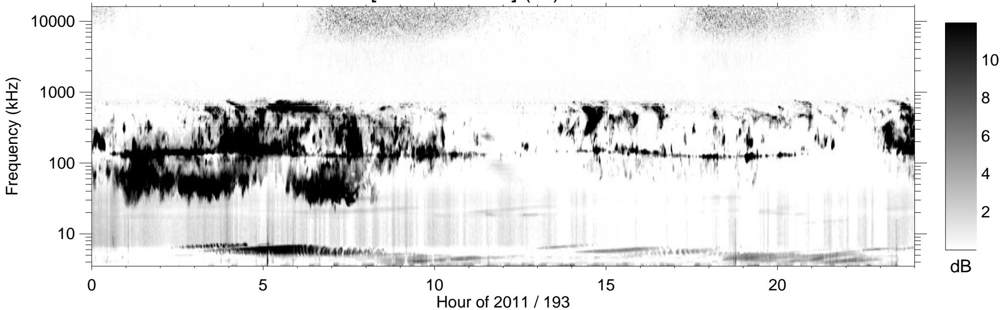
RPWS [ABCH1H2/Ex] (-B) 2011/07/12
