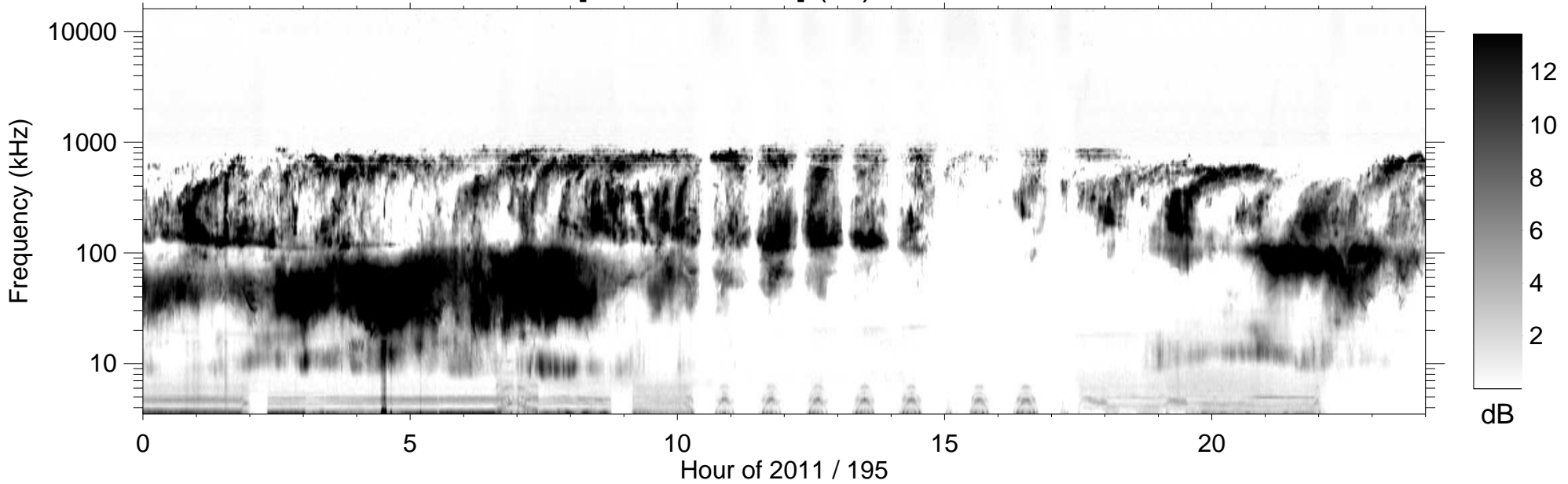
RPWS [ABCH1H2/Ex] (-B) 2011/07/14
