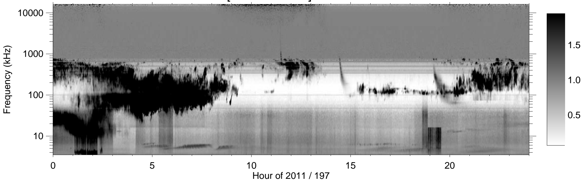
RPWS [ABCH1H2/Ex] (-B) 2011/07/16
