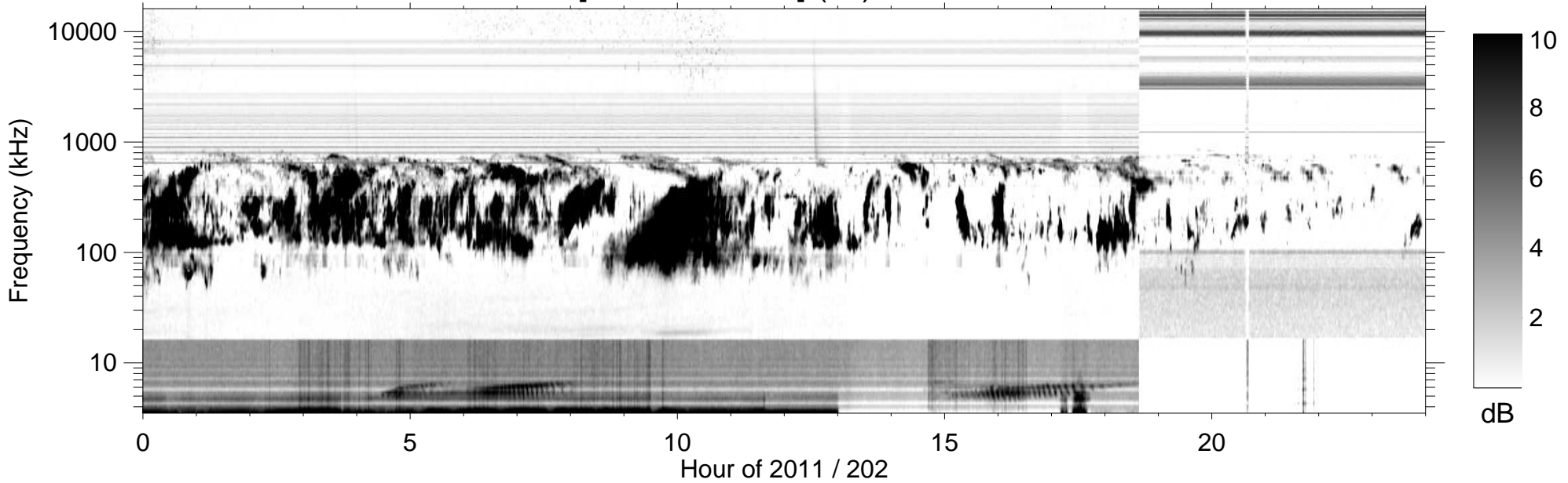
RPWS [ABCH1H2/Ex] (-B) 2011/07/21
