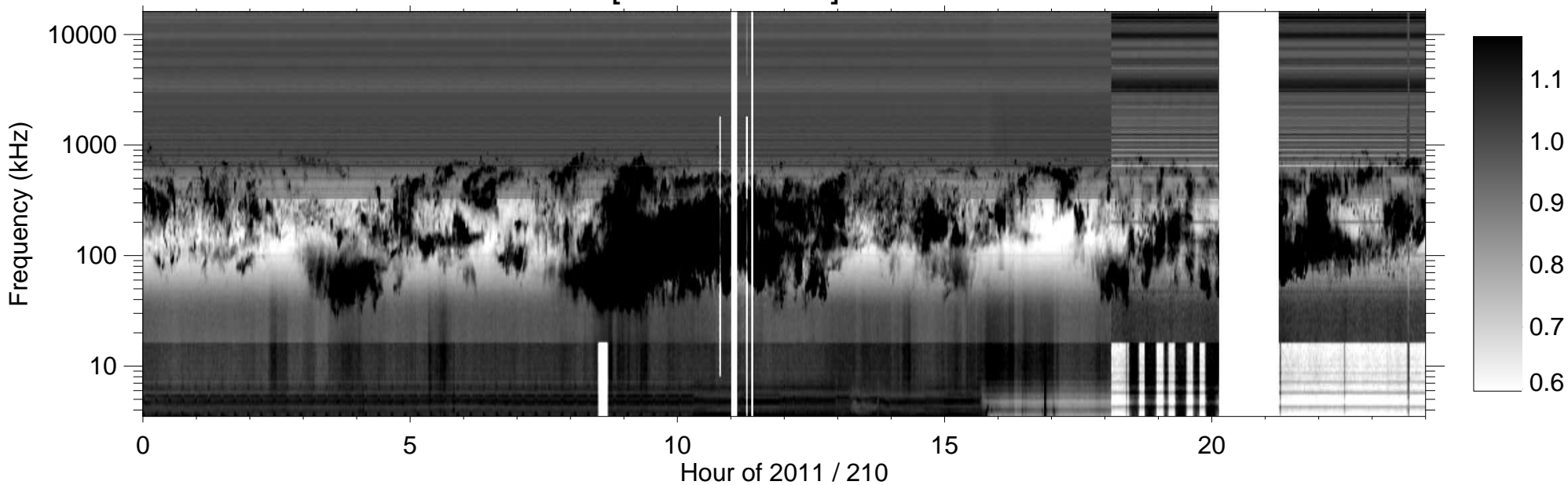
RPWS [ABCH1H2/Ex] (-B) 2011/07/29
