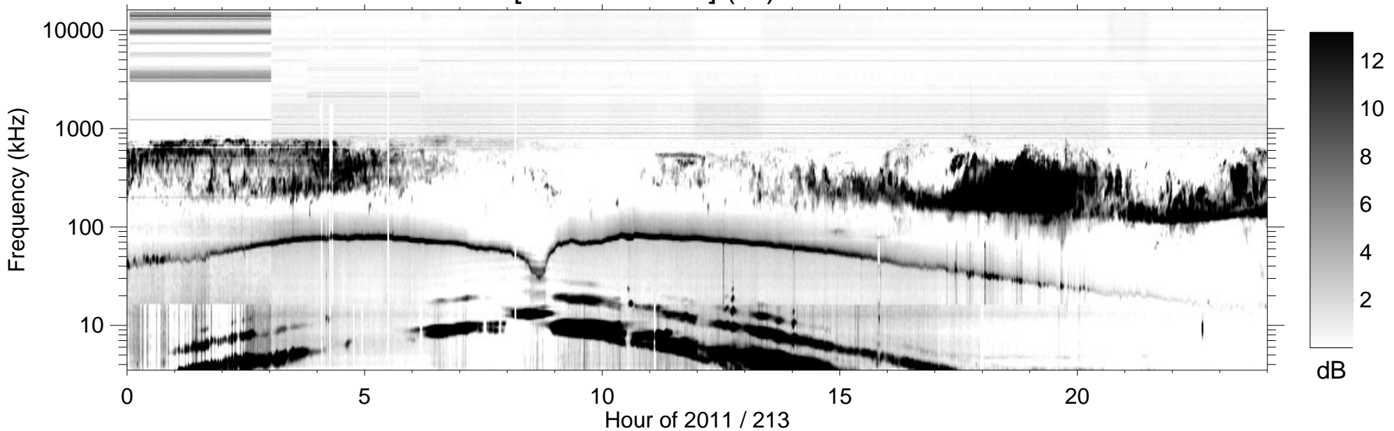
RPWS [ABCH1H2/Ex] (-B) 2011/08/01
