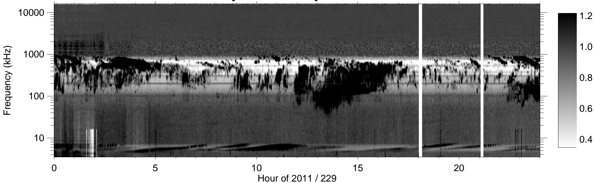
RPWS [ABCH1H2/Ex] (-B) 2011/08/17
