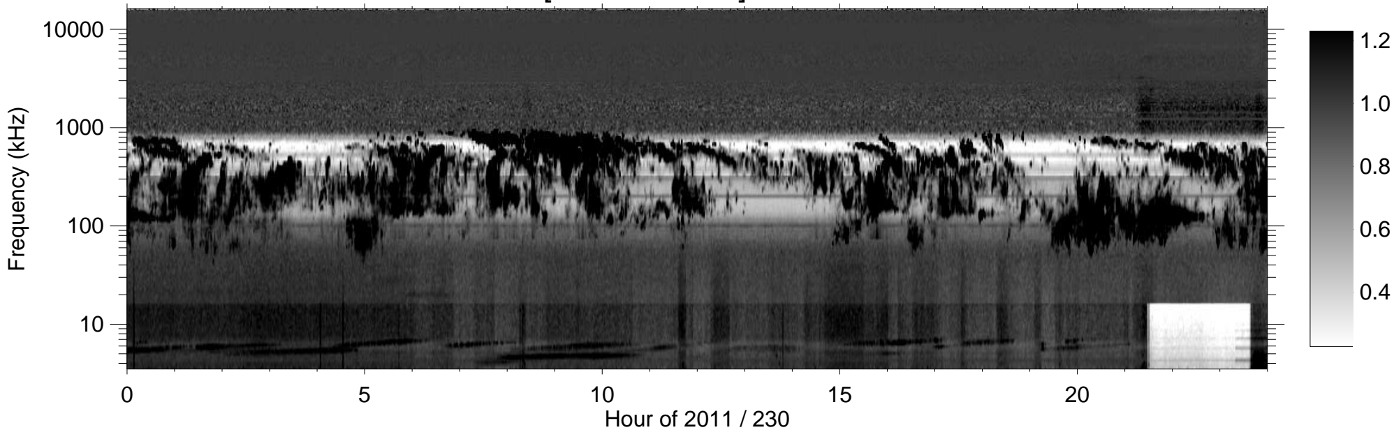
RPWS [ABCH1H2/Ex] (-B) 2011/08/18
