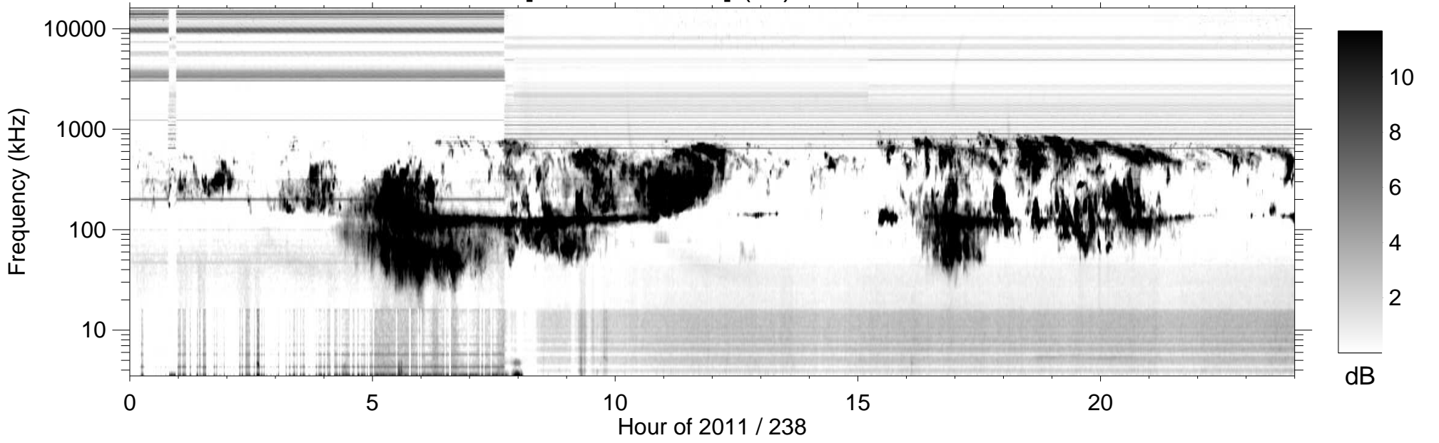
RPWS [ABCH1H2/Ex] (-B) 2011/08/26
