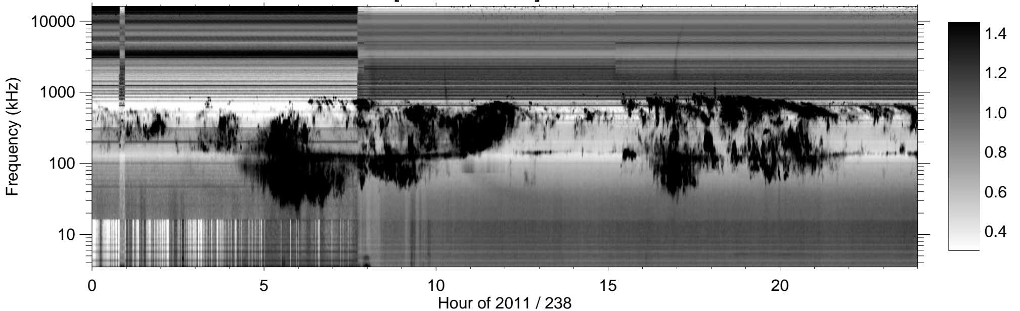
RPWS [ABCH1H2/Ex] (-B) 2011/08/26
