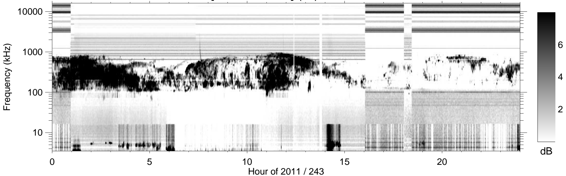
RPWS [ABCH1H2/Ex] (-B) 2011/08/31
